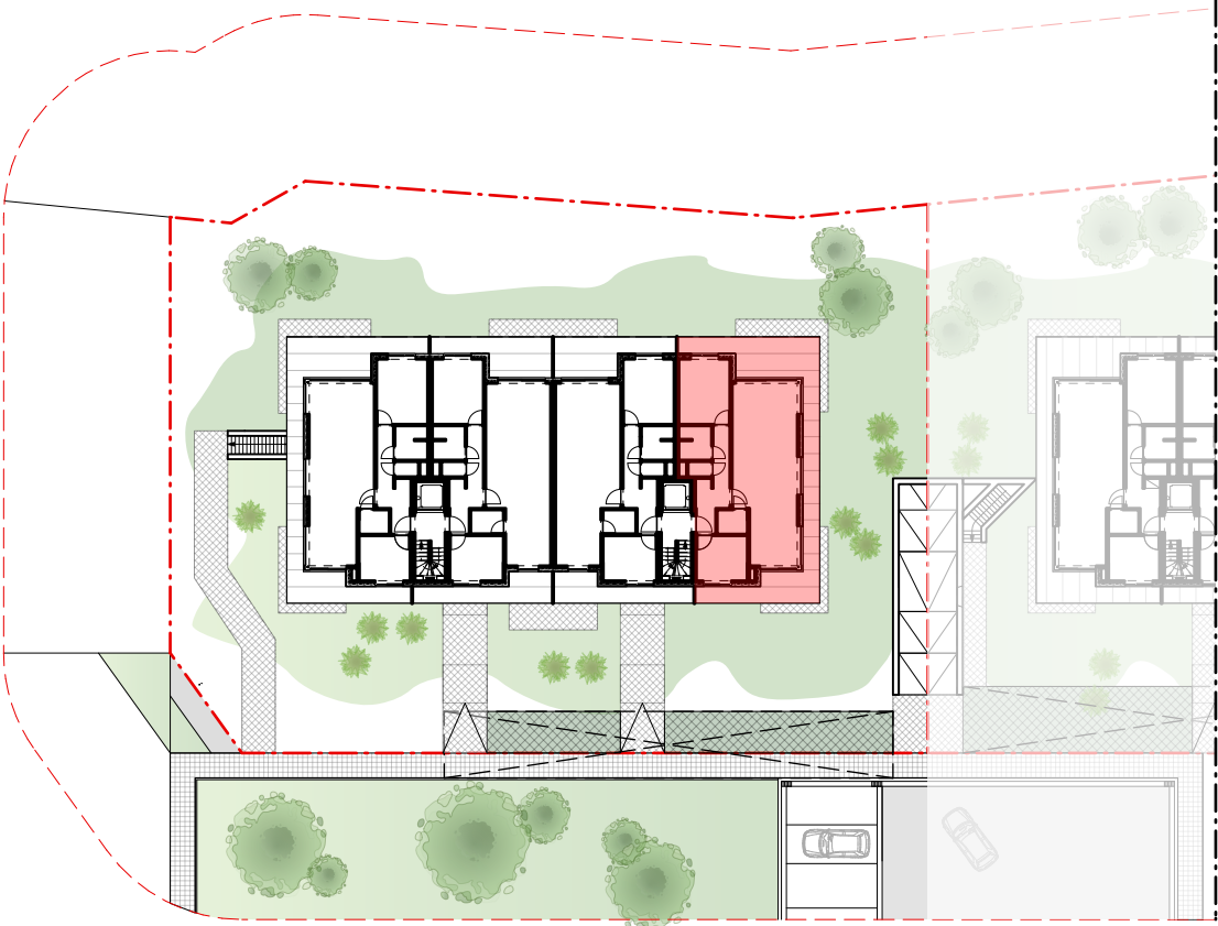
INPLANTINGSPLAN
